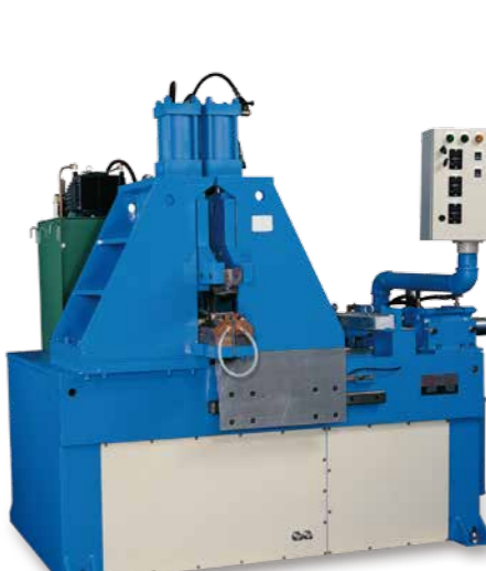
Pneumatic/Hydraulic Flash Butt Welding Machine Rated Capacity : 50~600 KVA 空油壓式閃焊·碰焊機
