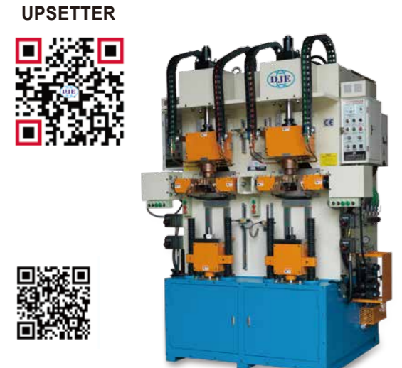
UPSETTER (Vertical Type Double Head) Electrical Heating Upsetter Rated Capacity : 16~650KVA Round Steel Dia : 6~60 mm 雙座電氣加熱擠壓鍛縮機
