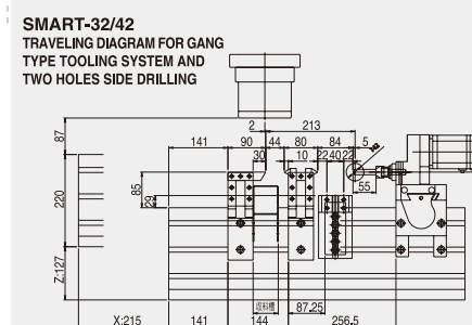
Gang Type
